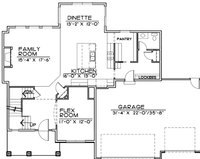
FIRST FLOOR • 1300 SQ.FT.
